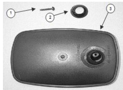
Figure 205: Dismantled mirror
