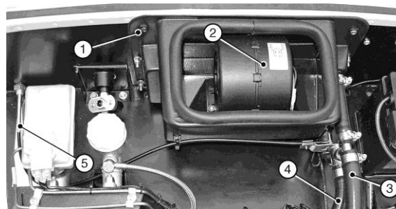
Figure 53: Heater installation
